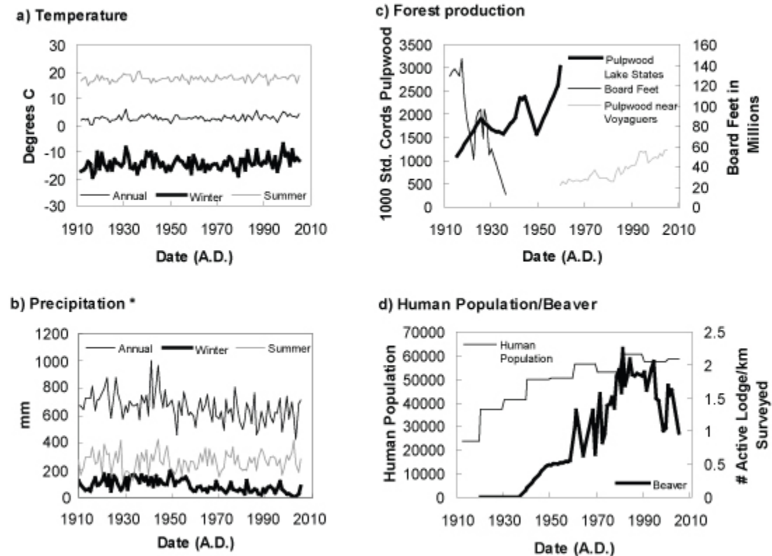
Figure II-2. Long-term data for the Voyageurs National Park region. Climate variables include (a) temperature and (b) precipitation records from Fort Frances, Ontario, and International Falls, Minnesota. Resource use variables include (c) forest production and (d) human population and beaver index.
