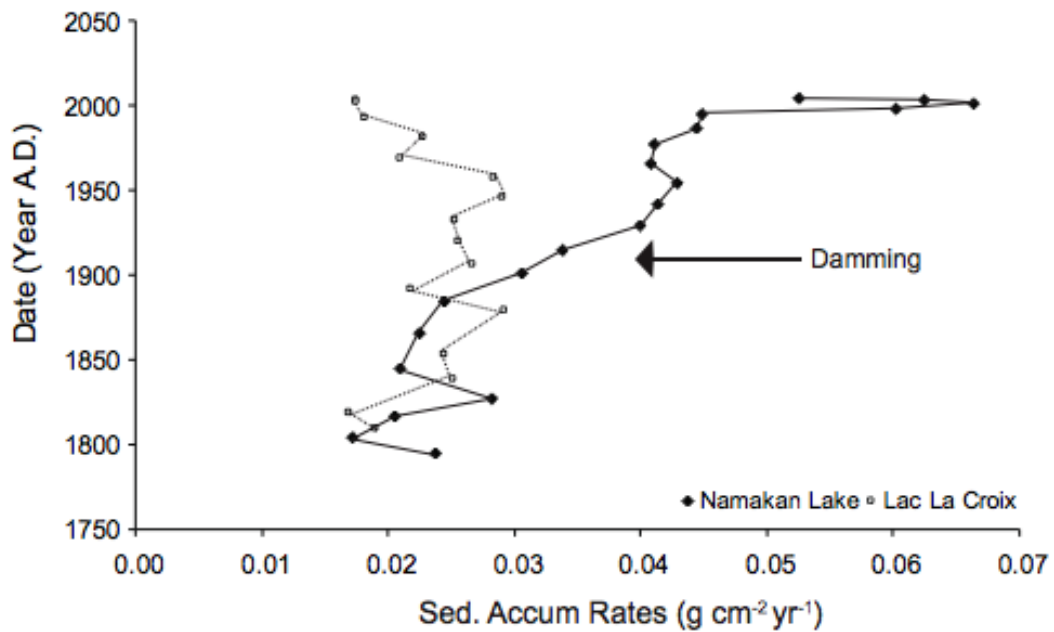
Figure I-4. Sediment accumulation rate through time in Namakan Lake and Lac La Croix. Note increased sediment accumulation rates in Namakan Lake after damming.
