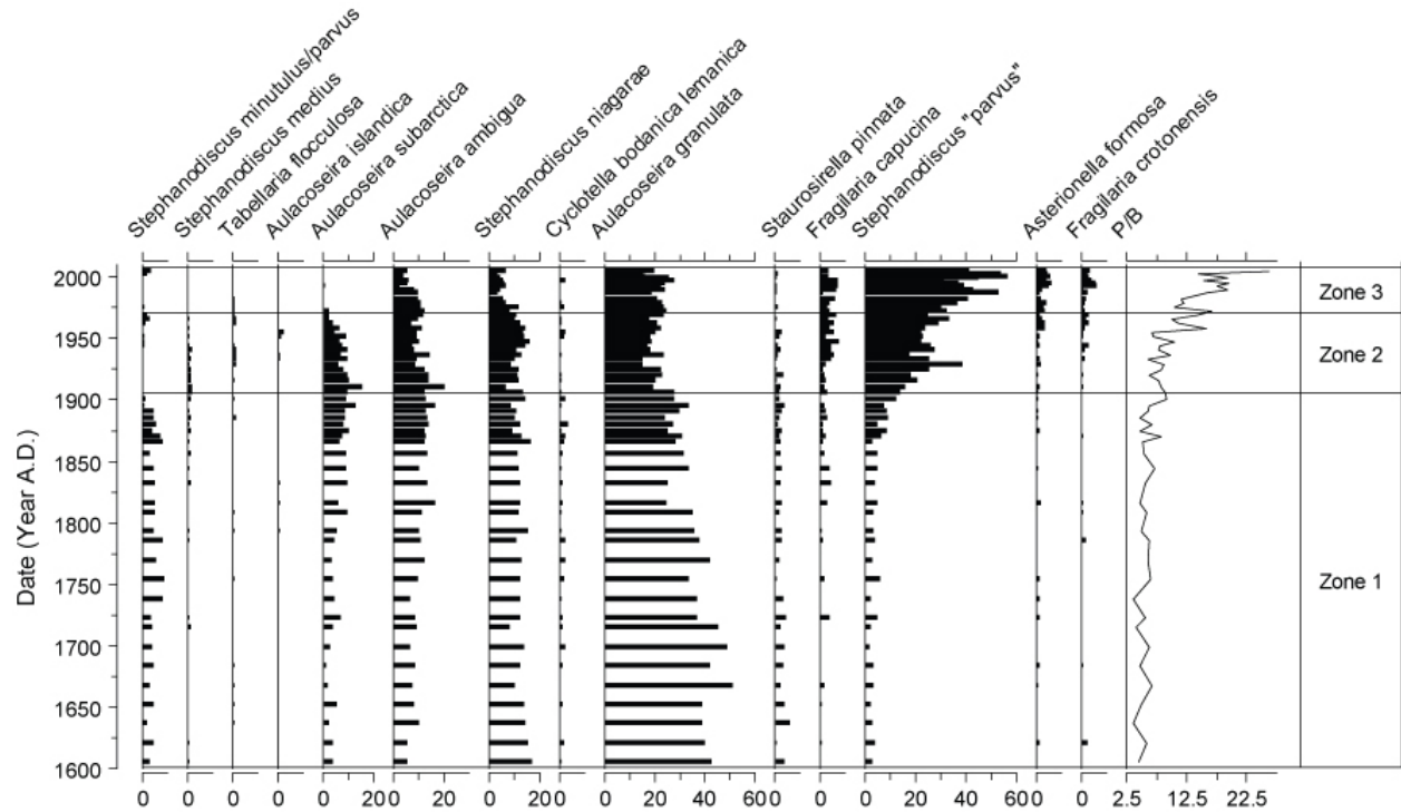
Figure II-8. Relative abundance of dominant diatom taxa and planktonic-to-benthic (P/B) ratio from Kabetogama Lake core, 1600–2005 A.D. Biostratigraphic zones as determined by CONISS denoted in right panel. Taxa occurred in at least one sample at \geq 2\% relative abundance.
