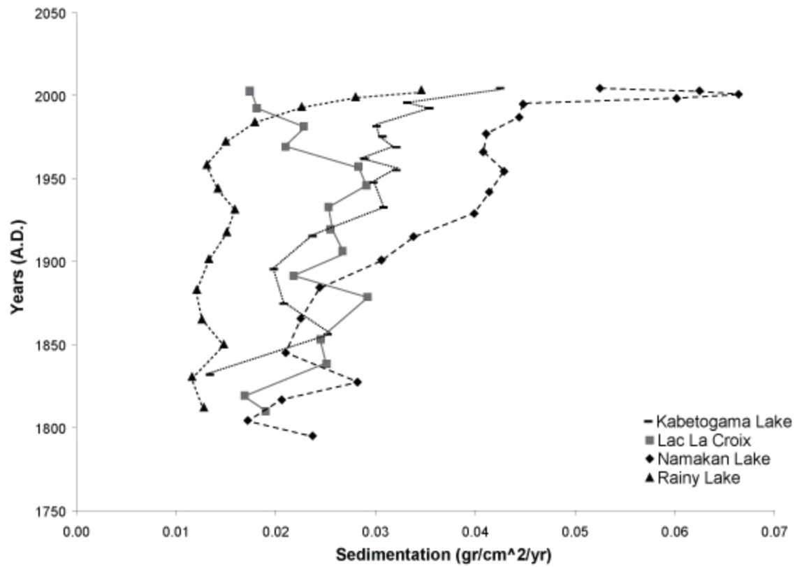
Figure II-6. Sediment accumulation rate ( \text{g cm}^{-2} \text{yr}^{-1} ) through time in Kabetogama Lake, Namakan Lake, Rainy Lake, and Lac La Croix. Note the increased sediment accumulation rates in Kabetogama Lake and Namakan Lake following damming, and post-1950s increases in Rainy Lake.
