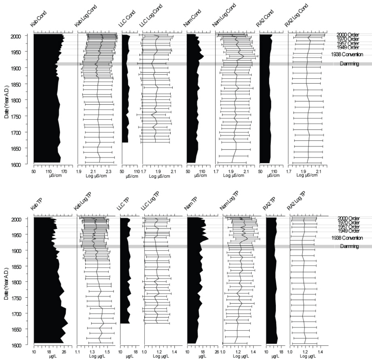
Figure II-13. Diatom-inferred conductivity (Cond) and total phosphorus (TP) reconstructions and model error estimates for Kabetogama Lake (KAB), Namakan Lake (NAM), Rainy Lake (RA2), and Lac La Croix (LLC). Damming and hydromanagement periods impacting Kabetogama Lake, Namakan Lake, and Rainy Lake are displayed in the right panel.
