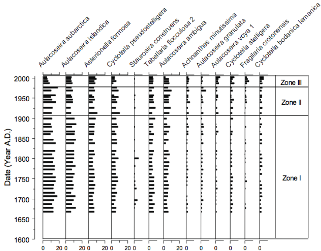
Figure I-7. Relative abundance of dominant diatom taxa from Lac La Croix, 1668–2005 A.D. See Figure I-6 for details.
