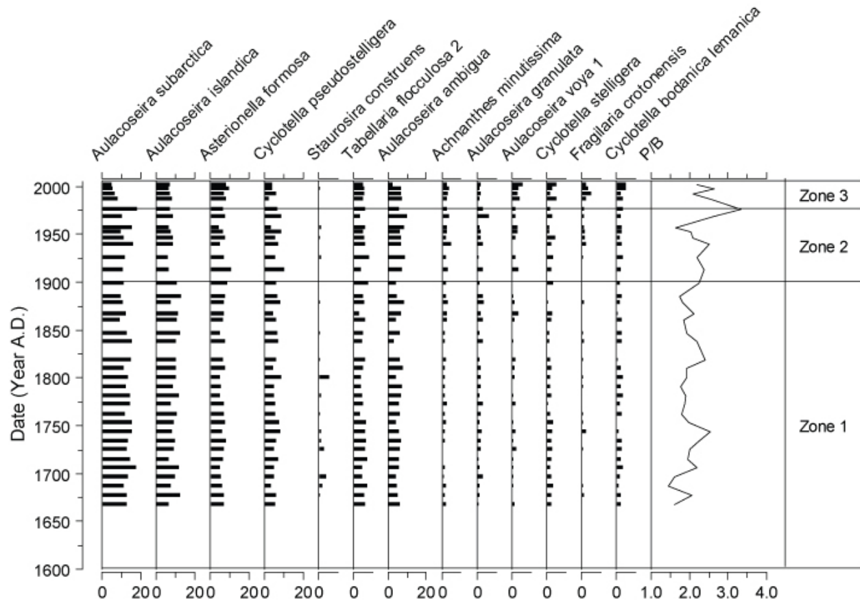
Figure II-11. Relative abundance of diatom taxa and P/B ratio from Lac La Croix, 1668–2005 A.D. See Figure II-8 for details.
