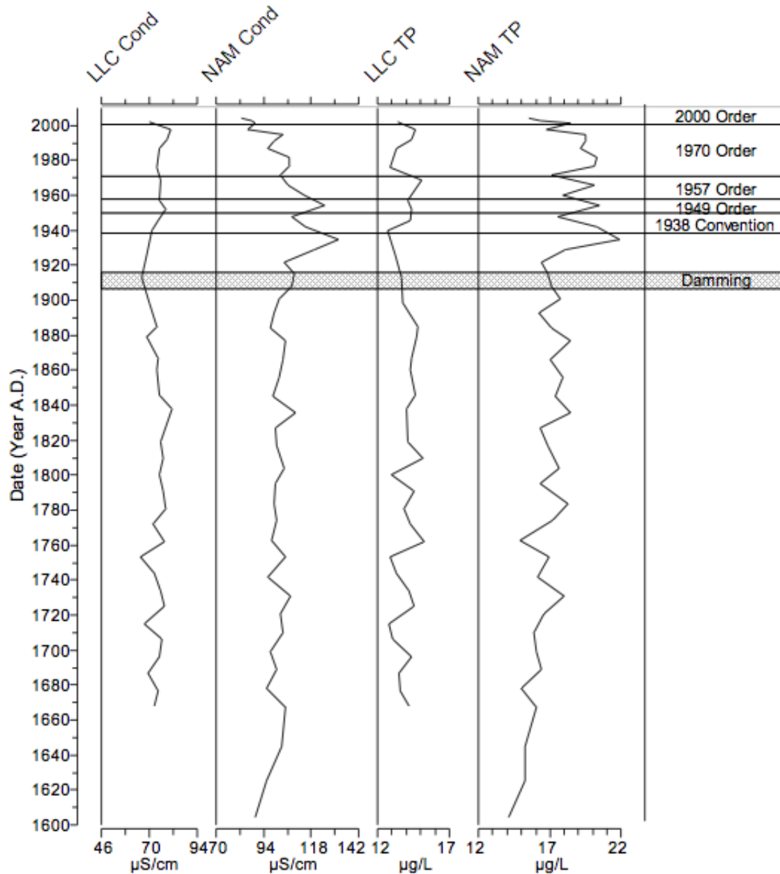
Figure I-9. Diatom-inferred conductivity (Cond) and total phosphorus (TP) reconstructions for Namakan Lake (NAM) and Lac La Croix (LLC). Damming and hydromanagement periods impacting Namakan Lake are displayed in the right panel.
