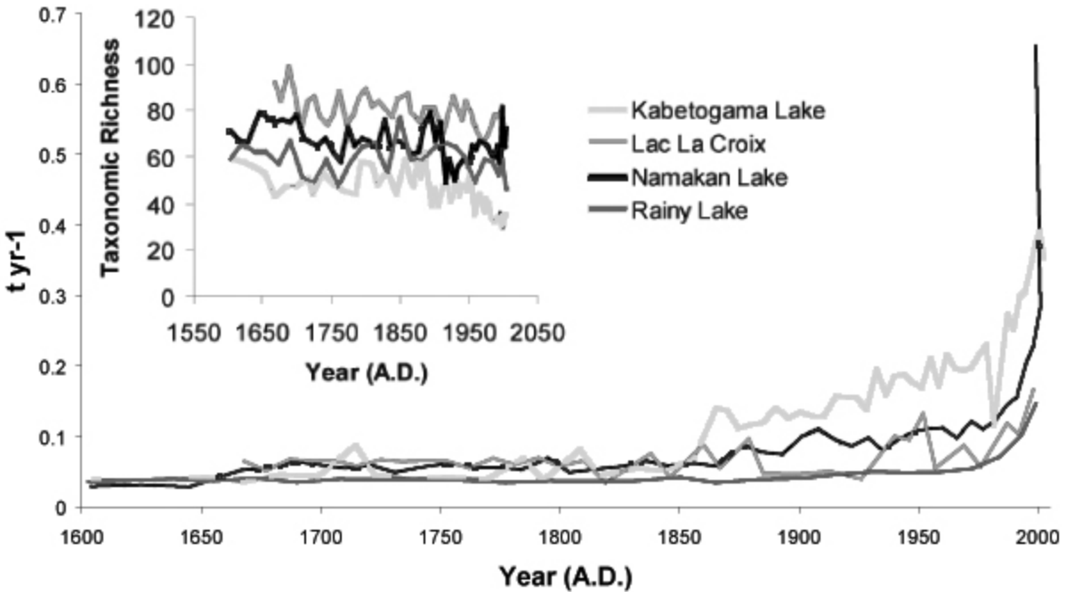
Figure II-7. Taxonomic richness (S) and species turnover (t) of diatoms in Kabetogama Lake, Namakan Lake, Rainy Lake, and Lac La Croix through time.
