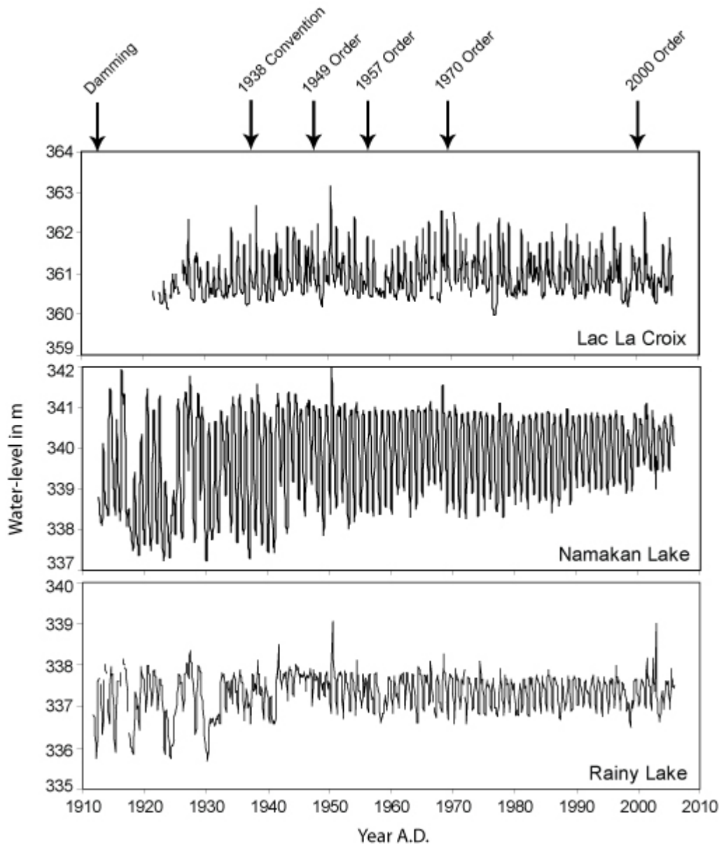
Figure II-3. Hydrograph of Namakan Lake at Kettle Falls (1912–2007), Rainy Lake at Fort Frances (1912–2007), and Lac La Croix at Campbell’s Camp (1921–2007). From Water Survey Canada (2007).
