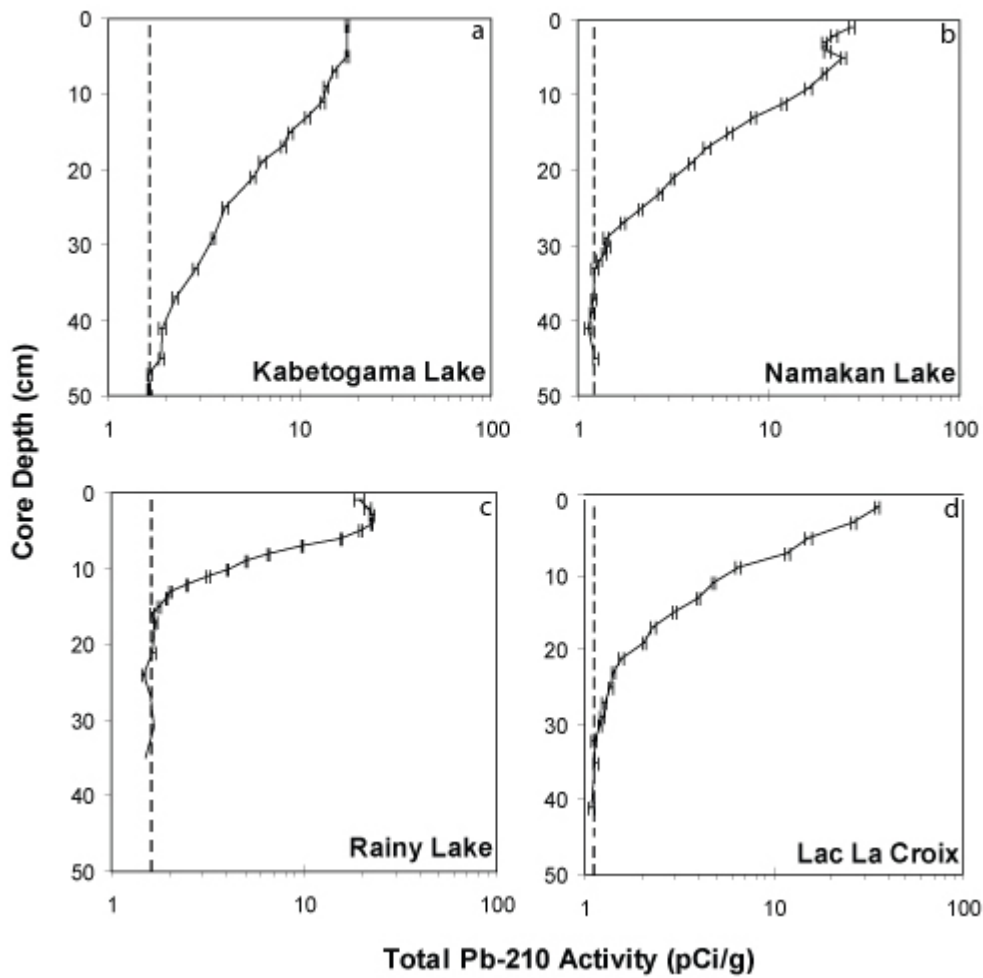
Figure II-4. Total ^{210}\text{Pb} inventory in sediment cores from Kabetogama Lake (a), Namakan Lake (b), Rainy Lake (c), and Lac La Croix (d) as a function of core depth based on the CRS model (Appleby and Oldfield 1978). Error bars represent \pm 1 s.d. propagated from counting uncertainty.
