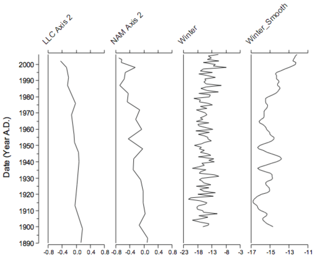
Figure I-10. Stratigraphic diagram comparing Axis 2 scores (see Figure I-8) based on Non-metric Multidimensional Scaling of down-core diatom communities from Namakan Lake (NAM) and Lac La Croix (LLC) against mean winter air temperature (°C) from Kenora, Ontario, Canada, and a locally weighted scatterplot smoothed (LOWESS) line of same with a span of 0.8. Note scale difference in two right panels.
