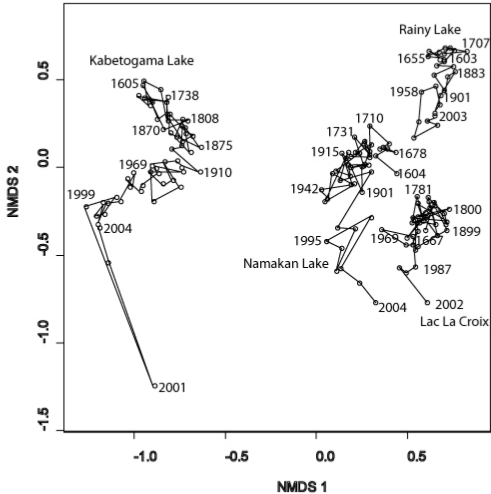
Figure II-12. Non-metric Multidimensional Scaling (NMS) analysis displaying dated samples from Kabetogama Lake, Namakan Lake, Rainy Lake, and Lac La Croix. Line segments connect samples in each core in chronological order.
