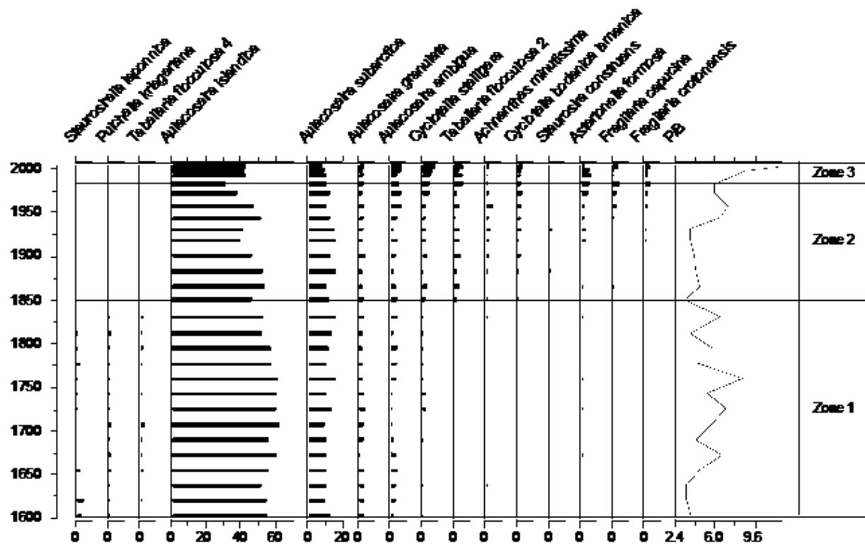
Figure II-10. Relative abundance of diatom taxa and P/B ratio from Rainy Lake core, 1600–2005 A.D. See Figure II-8 for details.
