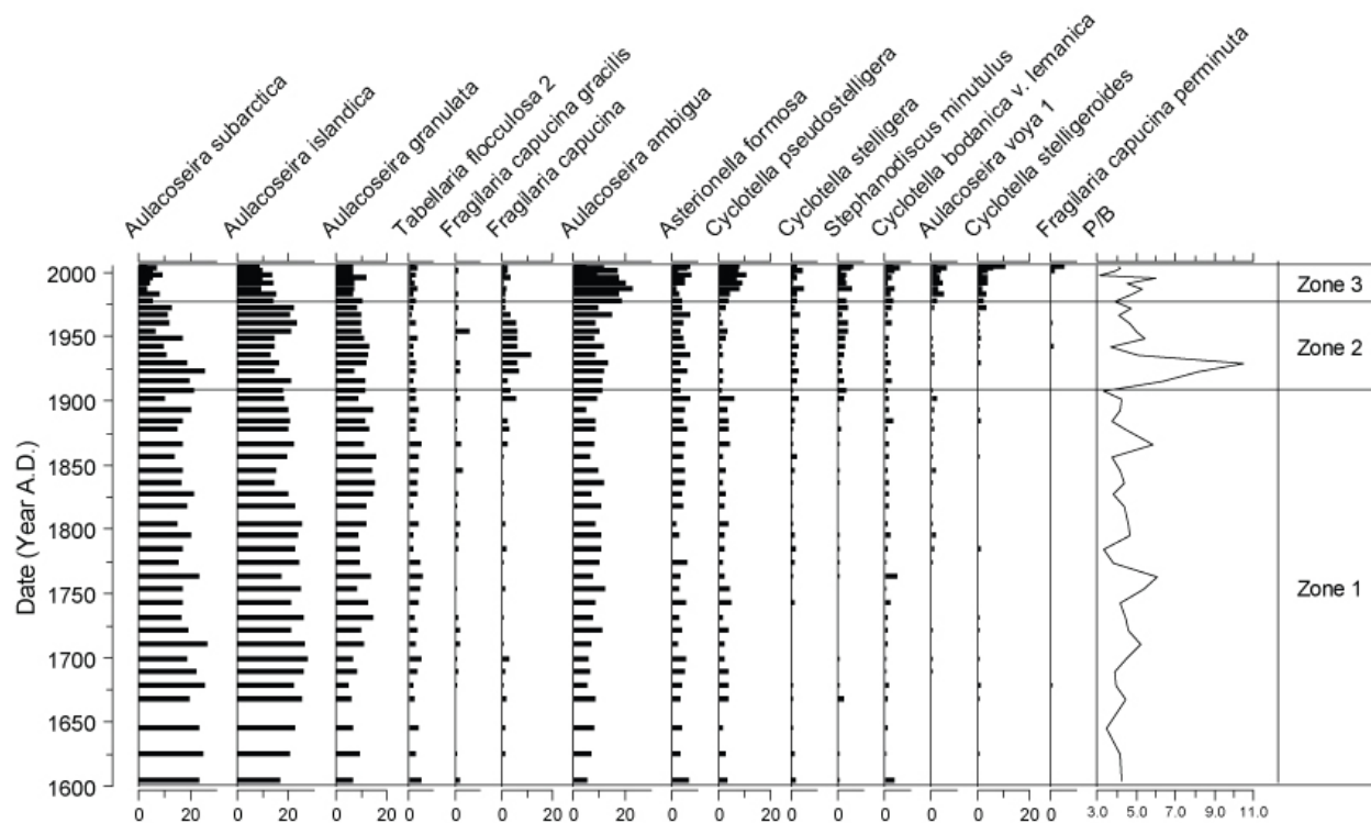
Figure II-9. Relative abundance of diatom taxa and P/B ratio from Namakan Lake core, 1600–2005 A.D. See Figure II-8 for details.
