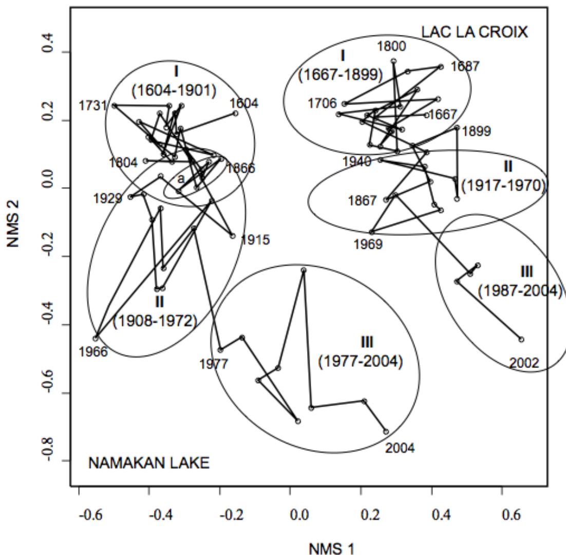
Figure I-8. Non-metric Multidimensional Scaling (NMS) analysis displaying dated samples from Namakan Lake and Lac La Croix. Line segments connect samples in each core in chronological order. Circled clusters of samples represent diatom biostratigraphic zones in each core identified using CONISS as first order and second order zones. Shifts between clusters represent periods of significant change in diatom communities.
