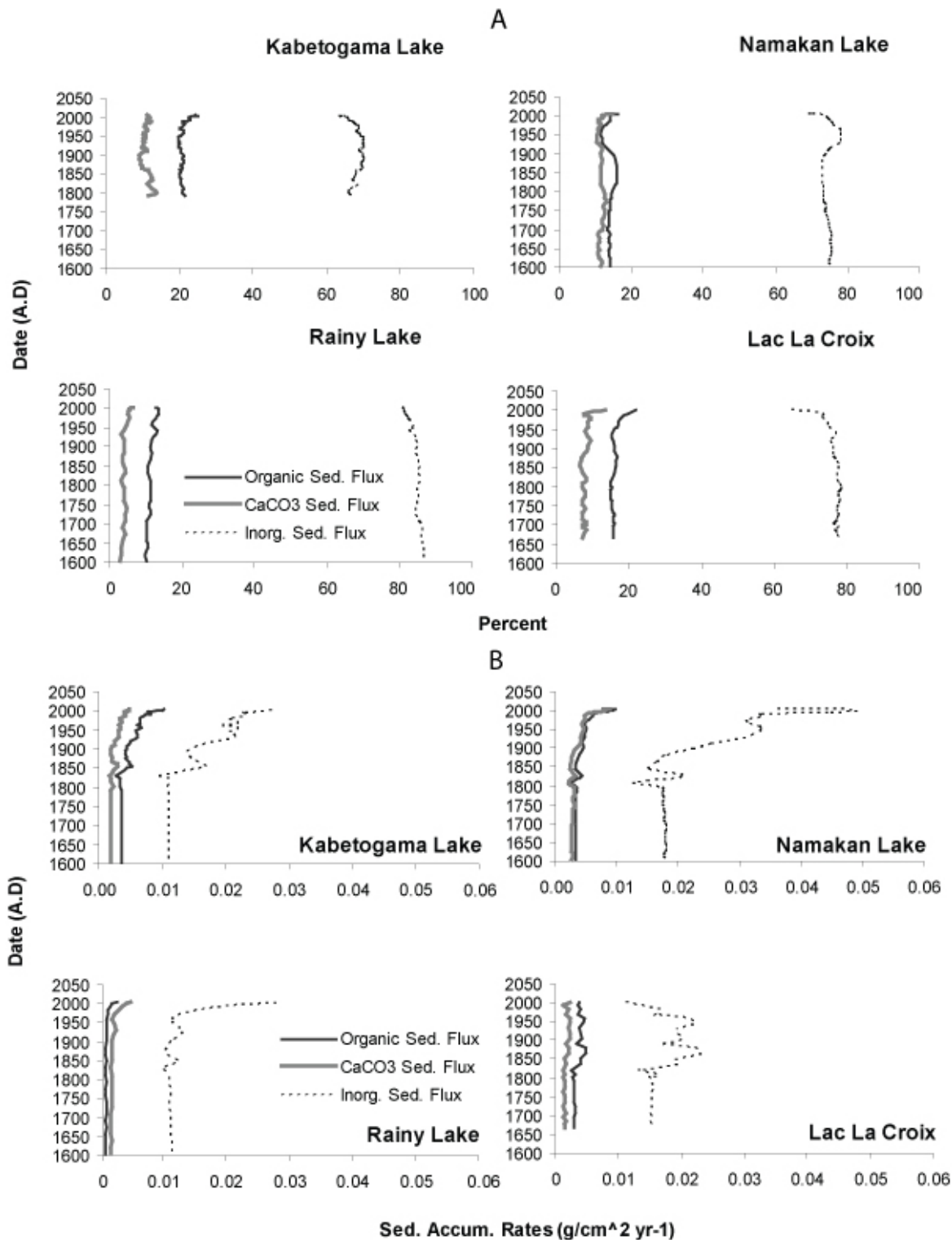
Figure II-5. (A) Inorganic, organic, and calcium carbonate content (dry weight percent) of Kabetogama Lake, Namakan Lake, Rainy Lake, and Lac La Croix sediments determined by loss-on-ignition. (B) Sediment flux of inorganics, organics, and carbonates ( \text{g cm}^{-2} \text{yr}^{-1} ) in Kabetogama Lake, Namakan Lake, Rainy Lake, and Lac La Croix.
