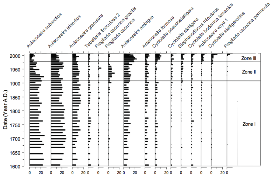
Figure I-6. Relative abundance of dominant diatom taxa from Namakan Lake core, 1600–2005 A.D. Biostratigraphic zones denoted in right panel. Taxa occurred in at least one sample at \leq 2\% relative abundance.
