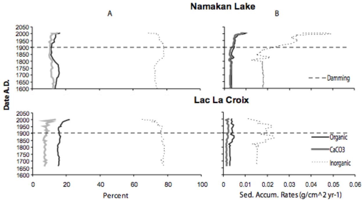
Figure I-3. Inorganic, organic, and calcium carbonate content of Namakan Lake and Lac La Croix sediments determined by loss on ignition (A), and sediment flux of inorganics, organics, and carbonated in Namakan Lake and Lac La Croix (B).
